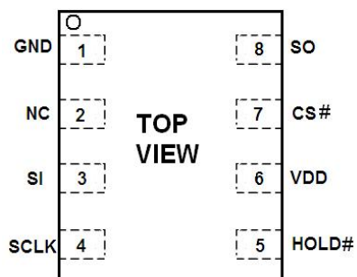
DFN8 2X3
