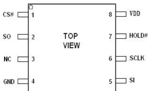
SOP-8
