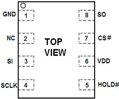
DFN8 2X3
